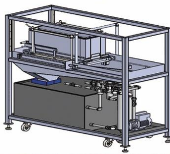
Washing Machine
